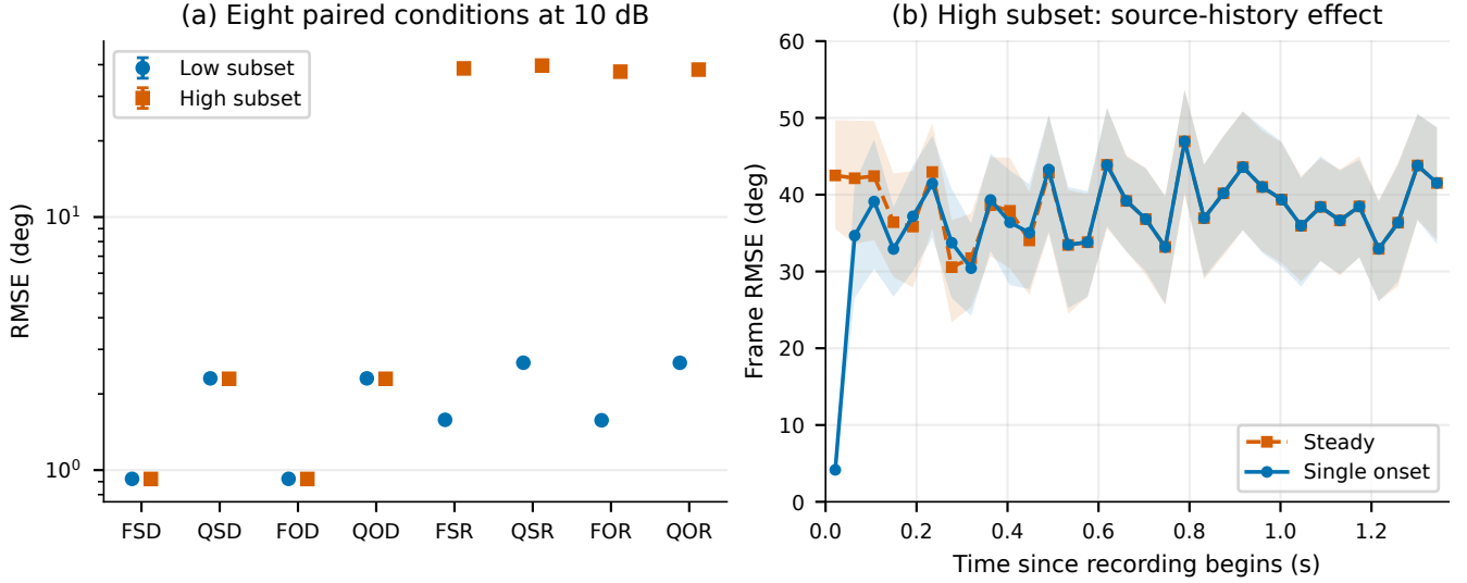
Figure 4. Arrival construction and source startup at 10 dB. (a) All eight combinations. F and Q denote fractional and rounded arrivals, S and O denote steady and onset histories, and D and R denote direct and reflected propagation. The low and high subsets contain 36 scenes each and differ in both array placement and wall absorption. Error bars and shaded bands are 95% intervals obtained by resampling complete recordings. (b) Matched fractional-arrival recordings with reflections in the high subset. In the steady condition, the source was already running when acquisition began. Markers indicate frame midpoints after the start of analysis.
