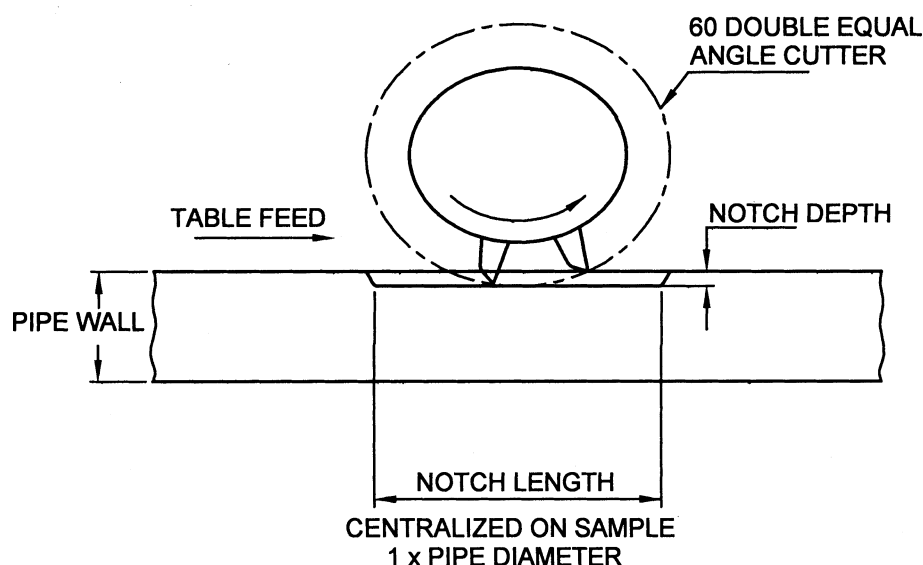
FIG. 8 NOTCH METHOD
