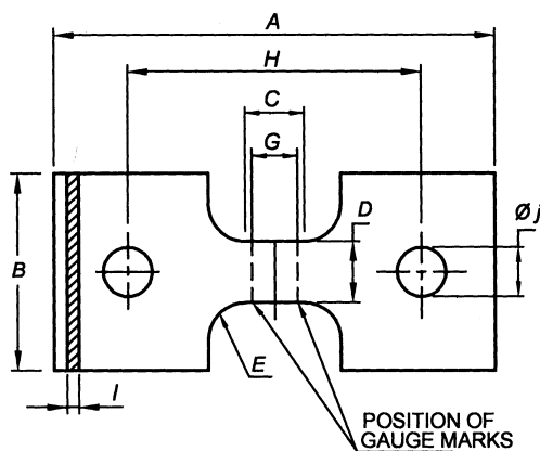
FIG. 6 TYPE 3 TEST PIECE
