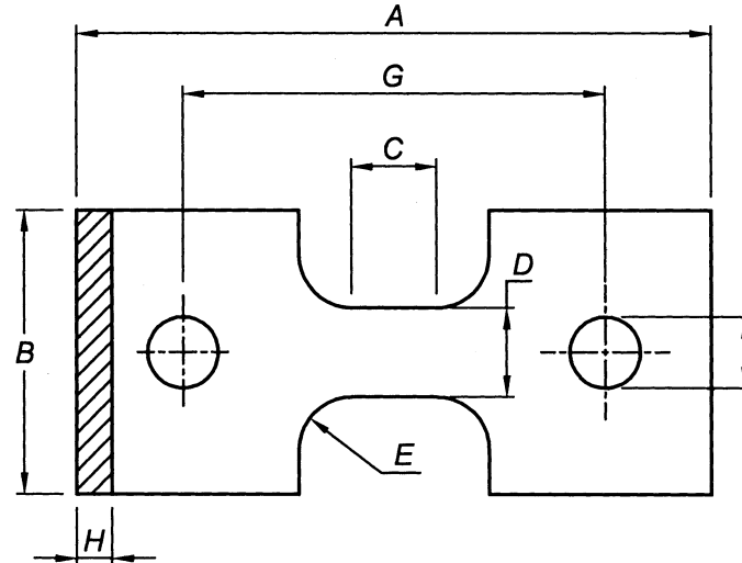
FIG. 2 MACHINED TYPE A TENSILE TEST PIECE (FOR E < 25 mm)
