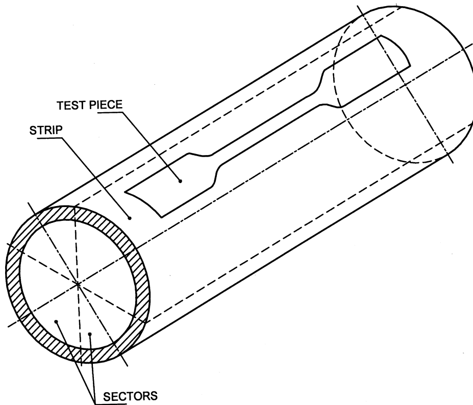
FIG. 7 PREPARATION OF TEST PIECES
