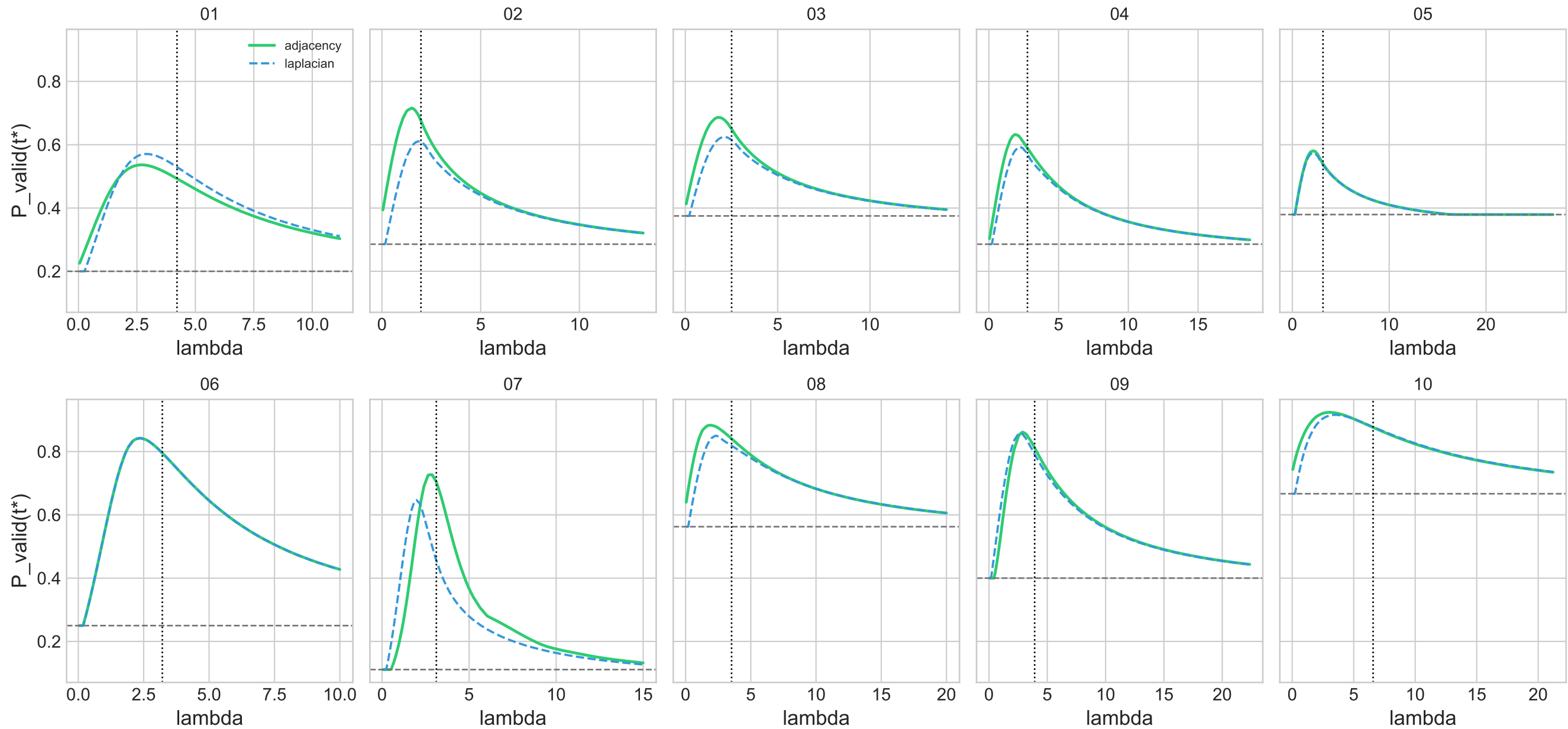
All lambda scans — adjacency and Laplacian conventions
