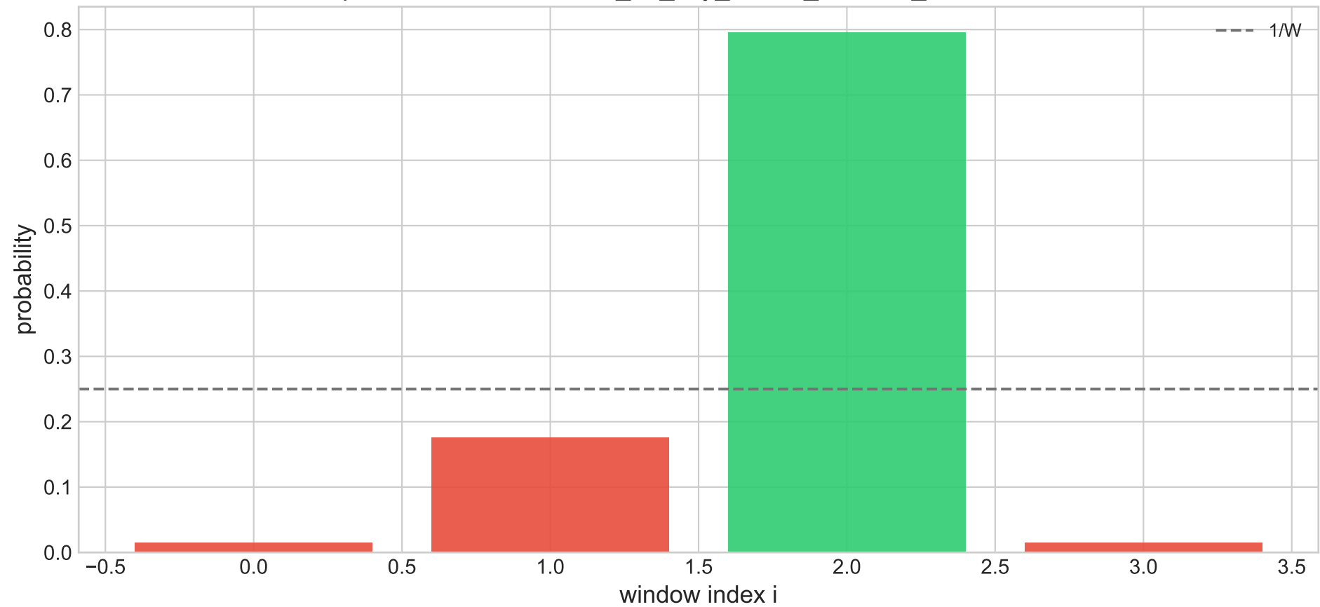
Optimal distribution — 06_2d_tiny_corner_block, P_valid=0.7953
