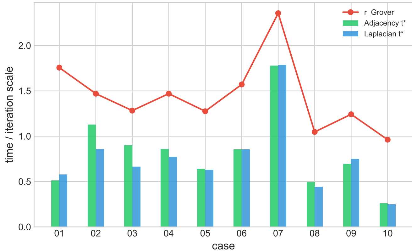
Time: adjacency vs Laplacian
