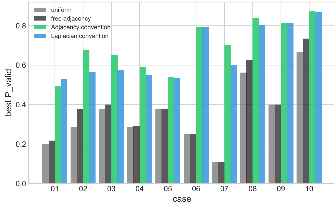
Probability: adjacency vs Laplacian
