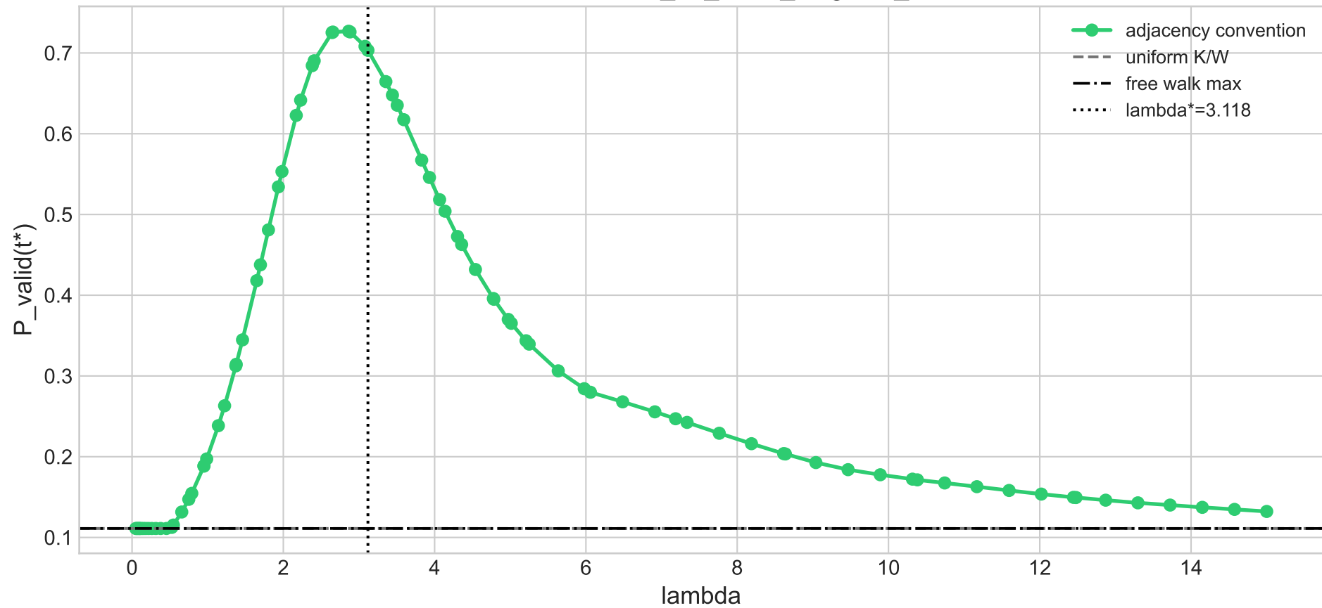
Lambda scan — 07_2d_small_diagonal_block
