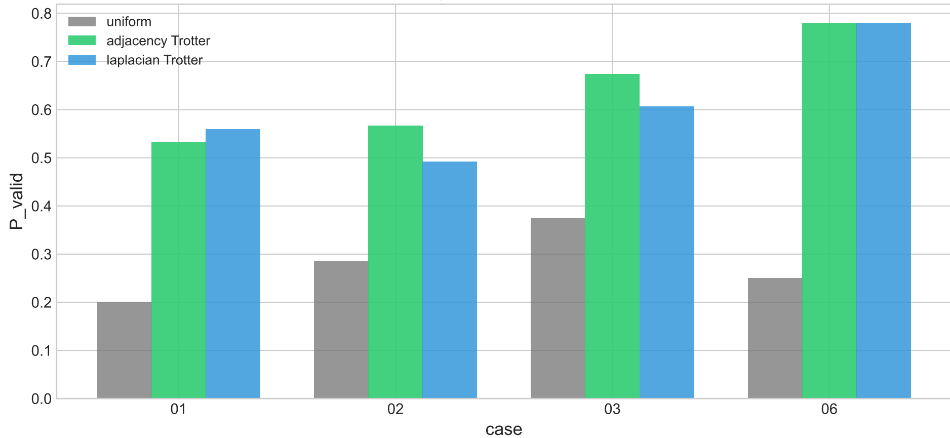
V7.1 hardware-ready Trotter QW: small-case simulation
