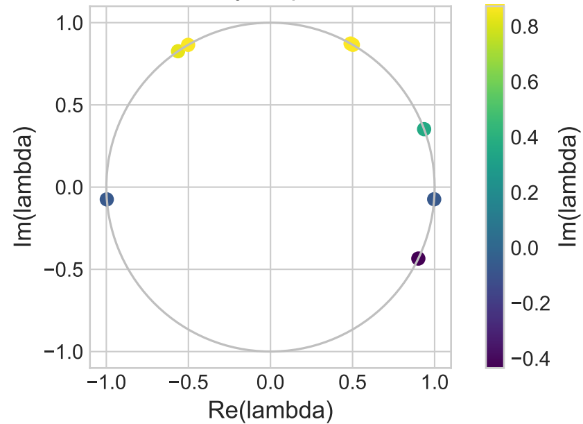
One-layer spectrum
