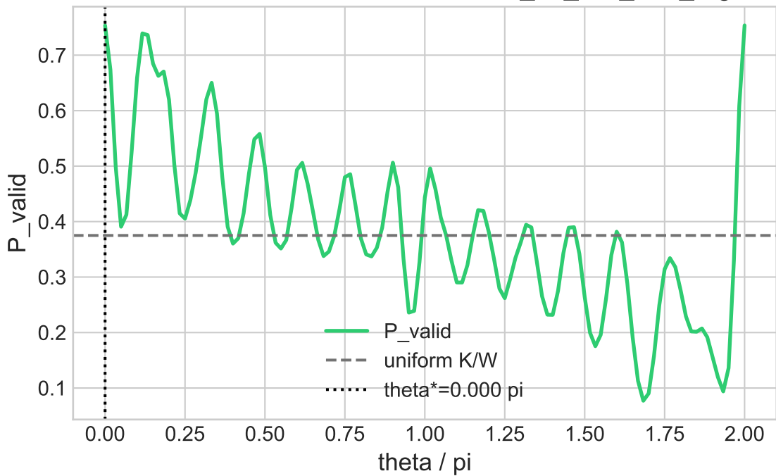
V4 theta scan at beta=0.300, r=14 - 03_1d_two_free_regions
