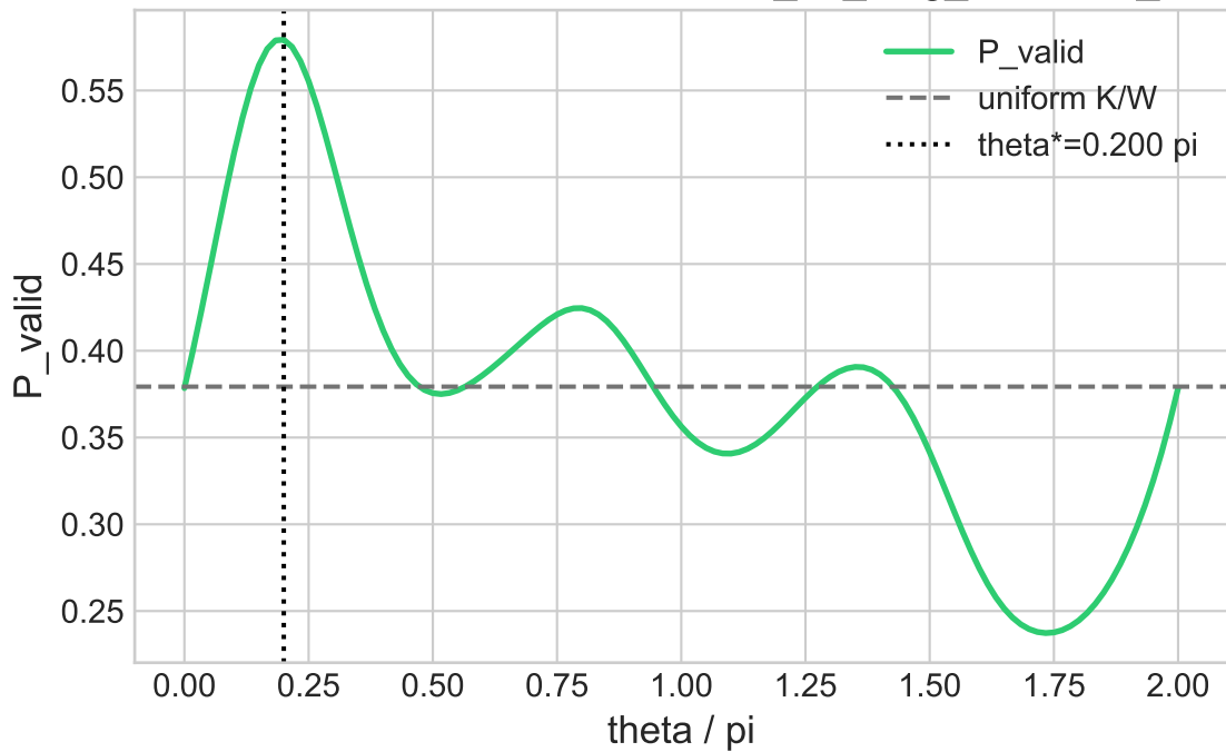
V4 theta scan at beta=0.180, r=3 - 05_1d_long_clustered_blocks
