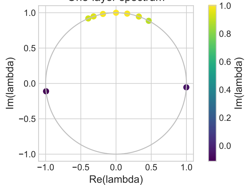
One-layer spectrum
