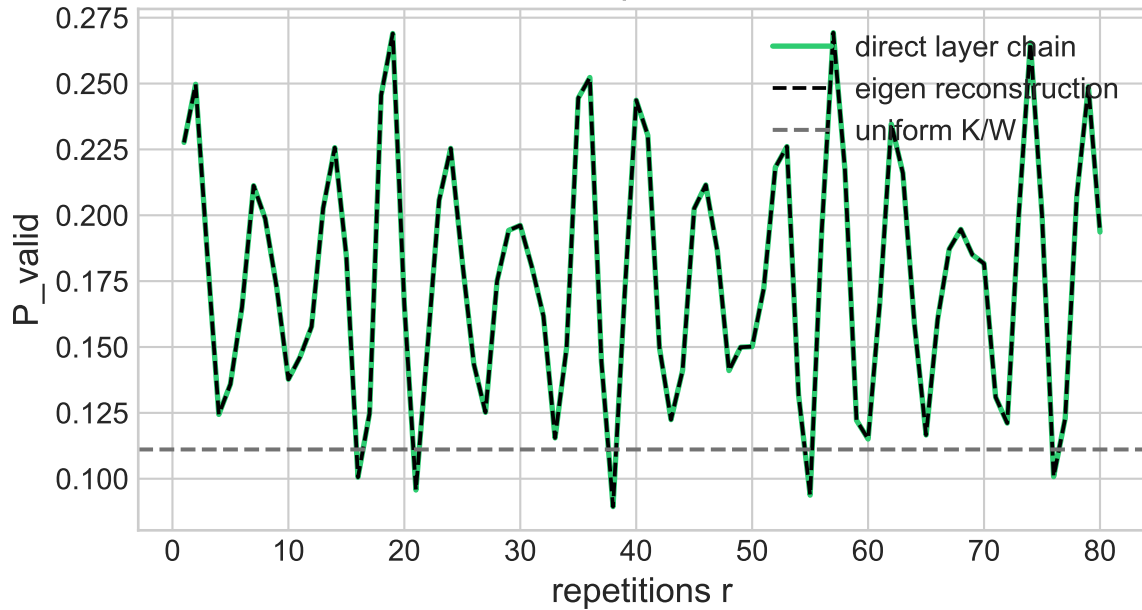
Period prediction
