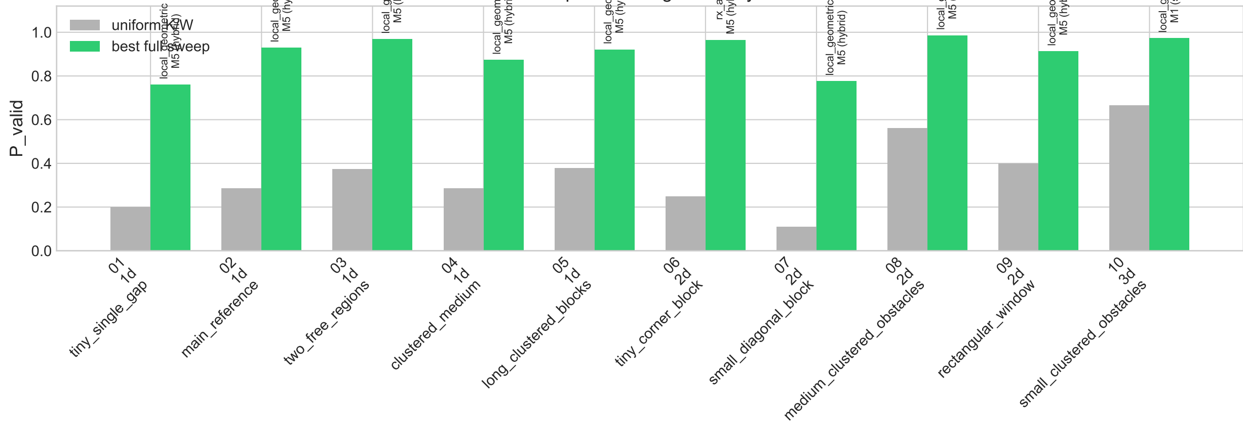
V4 full sweep best configuration by use case
