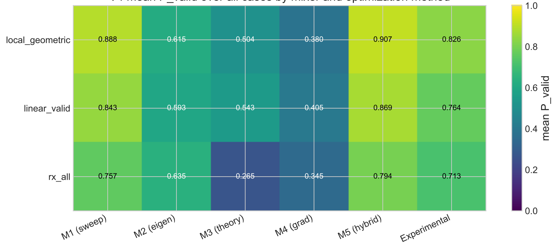
V4 mean P_valid over all cases by mixer and optimization method
