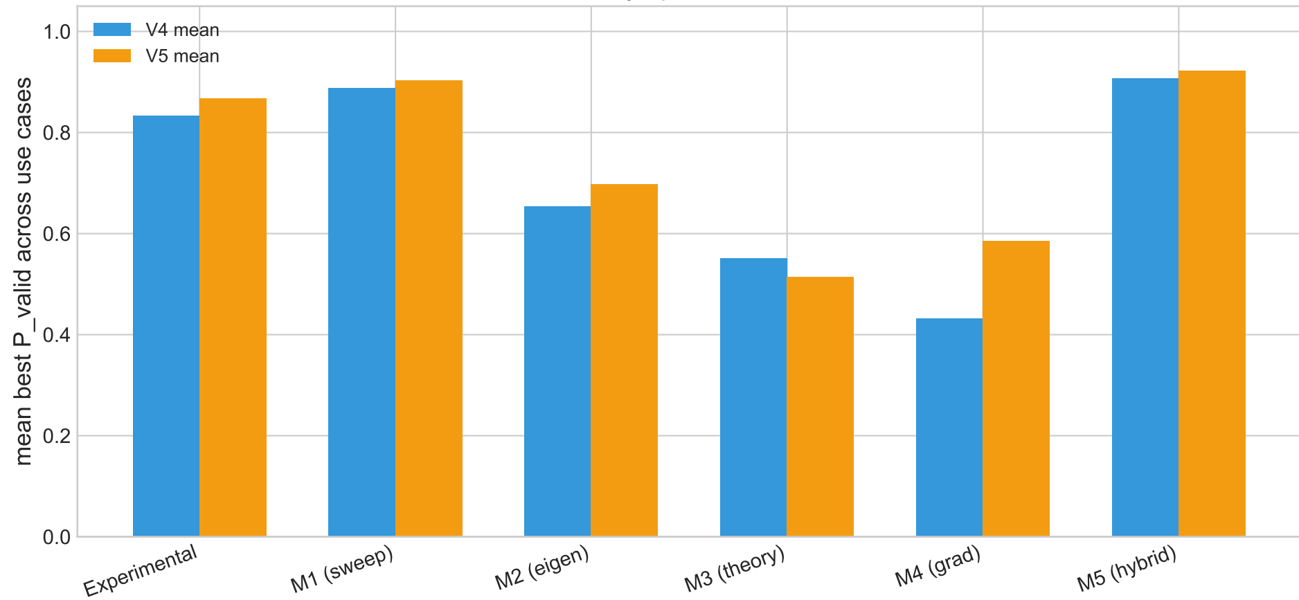
V4 vs V5 by optimization method
