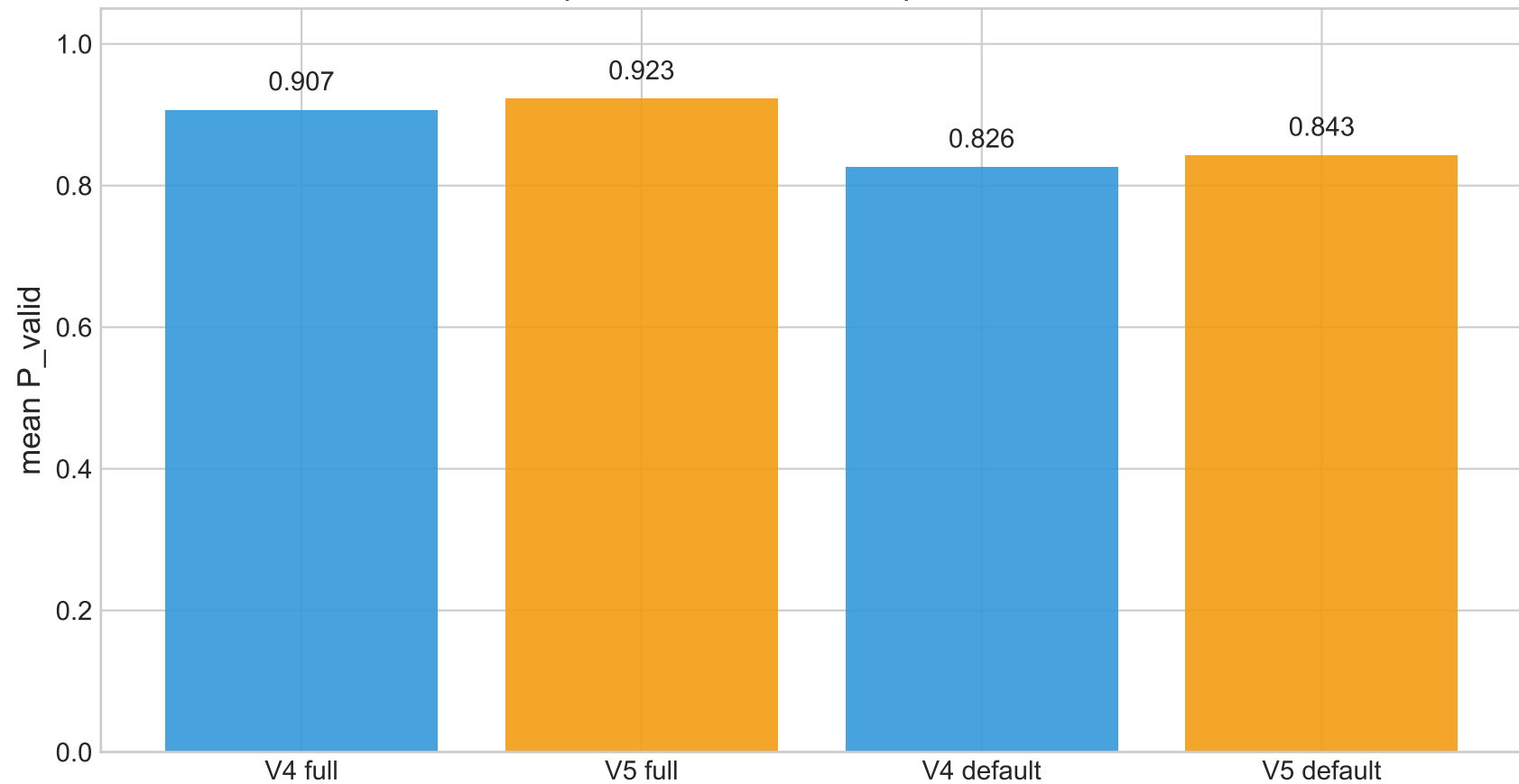
Overall V4 vs V5 performance: full sweep vs default-mixer reference
