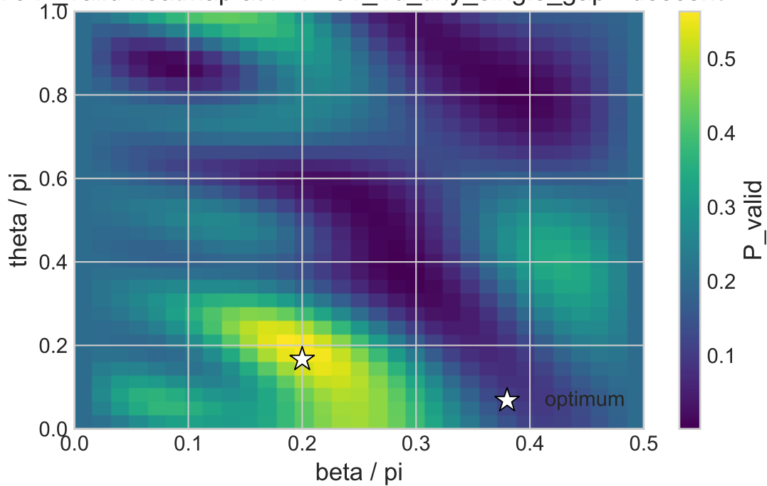
V5 P_valid heatmap at r=4 - 01_1d_tiny_single_gap - descent
