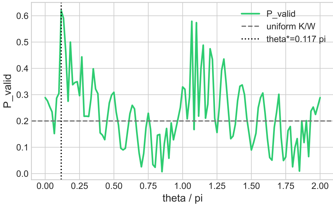
V5 theta scan at beta=0.300, r=57 - oriented_valid
