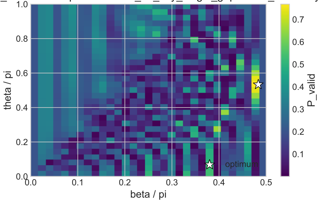
V5 P_valid heatmap at r=56 - 01_1d_tiny_single_gap - valid_boundary
