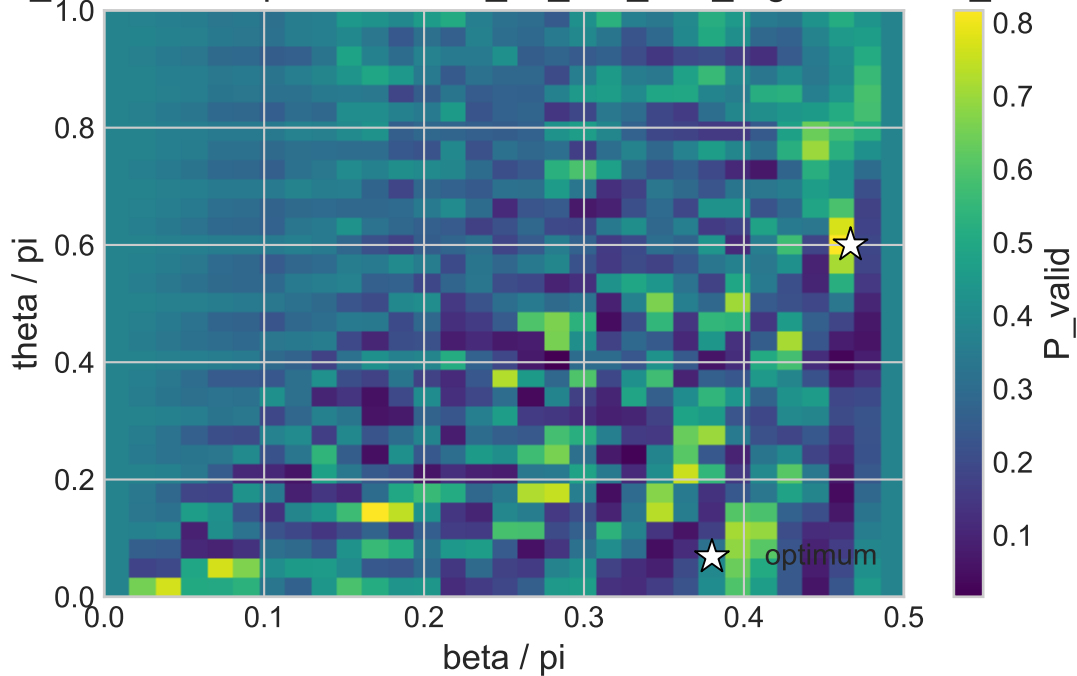
V5 P_valid heatmap at r=39 - 03_1d_two_free_regions - delta_cost
