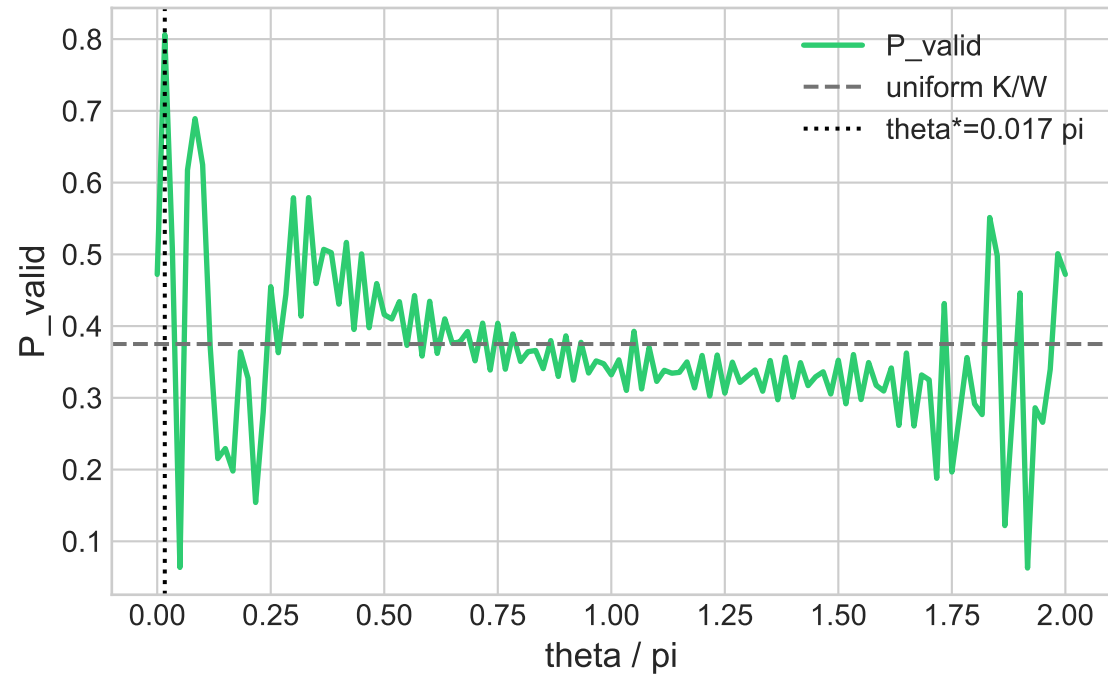
V5 theta scan at beta=0.300, r=54 - descent
