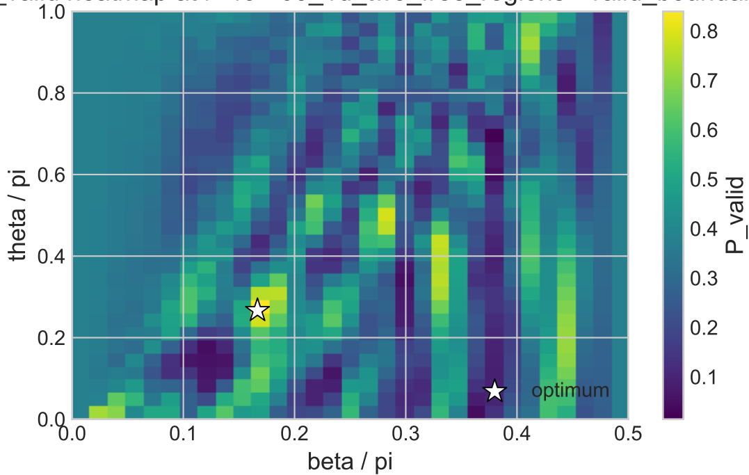
V5 P_valid heatmap at r=45 - 03_1d_two_free_regions - valid_boundary
