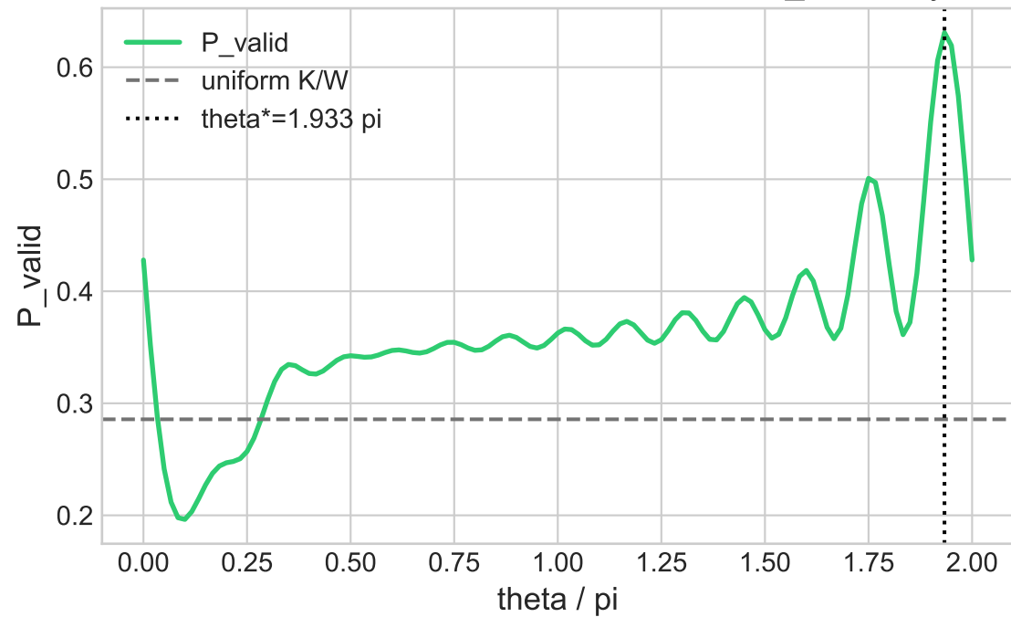
V5 theta scan at beta=0.240, r=14 - valid_boundary
