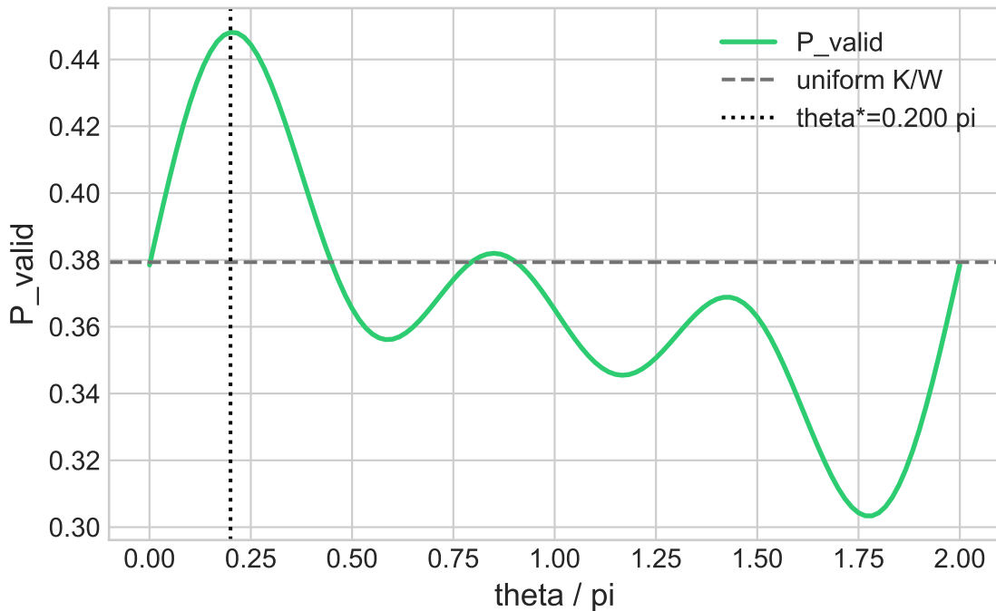
V5 theta scan at beta=0.180, r=3 - descent
