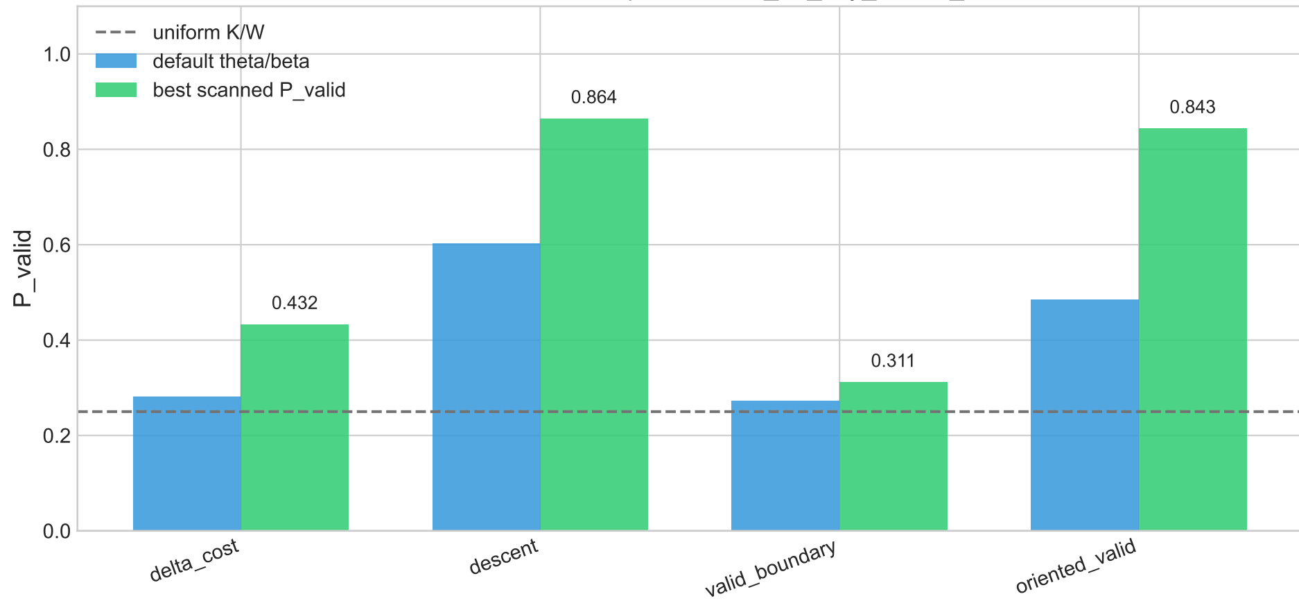
V5 transition mode comparison - 06_2d_tiny_corner_block
