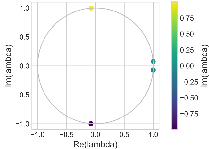
One-layer spectrum
