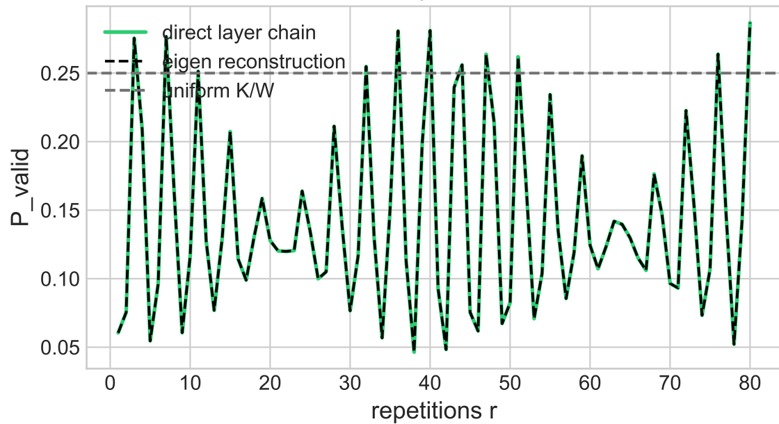
Period prediction
