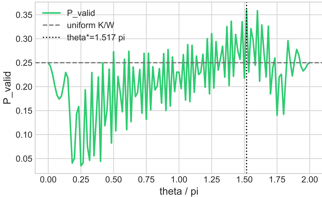
V5 theta scan at beta=0.280, r=57 - valid_boundary
