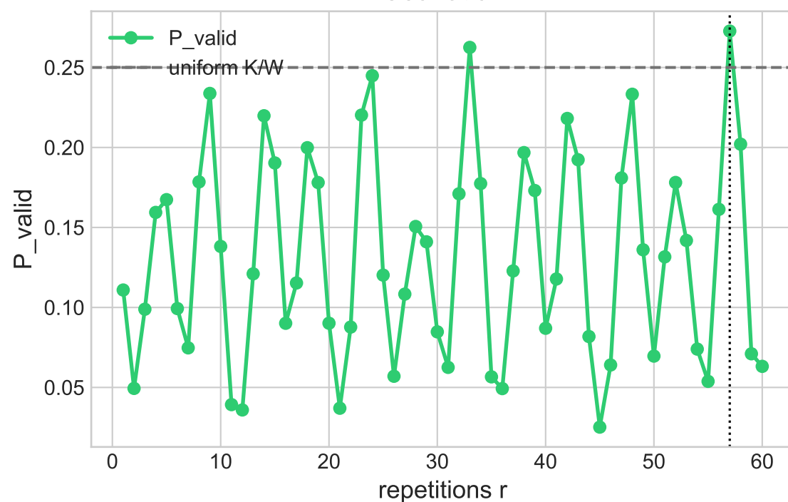
Theta scan
