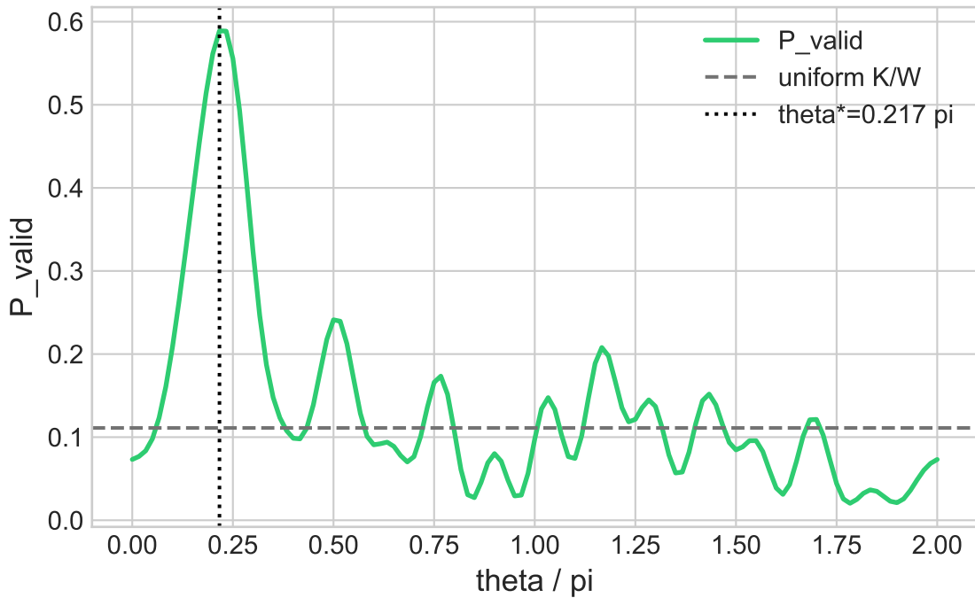
V5 theta scan at beta=0.240, r=8 - oriented_valid
