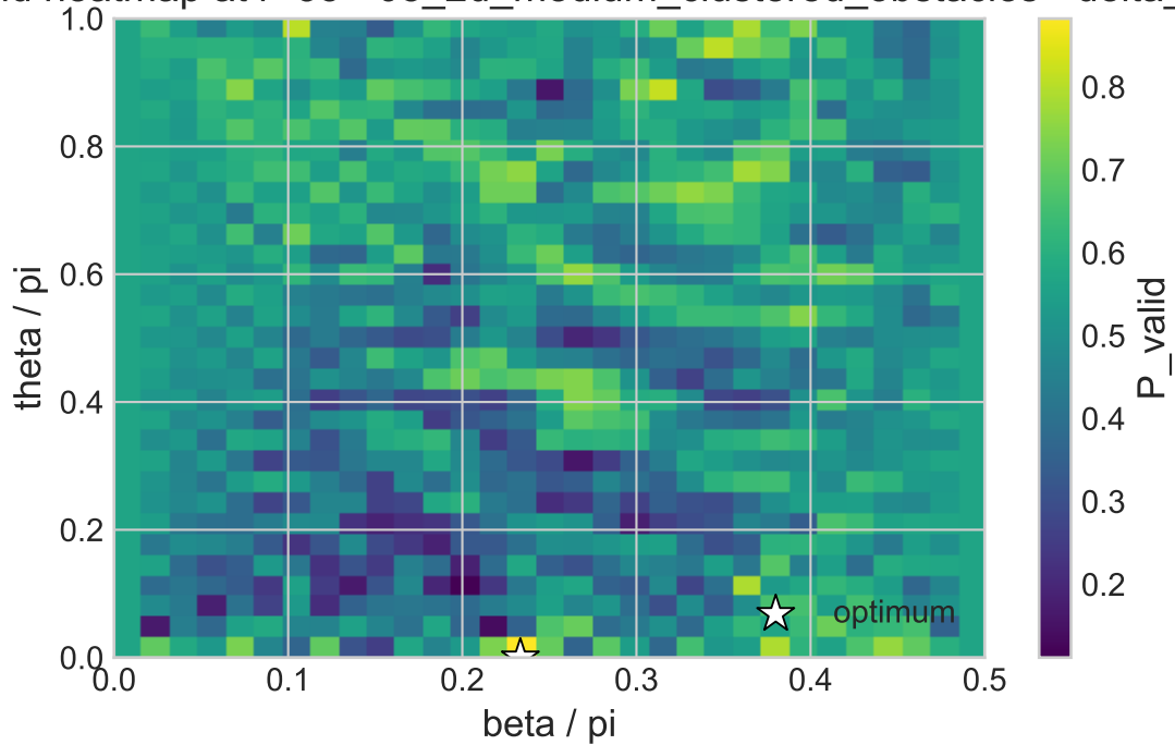
V5 P_valid heatmap at r=35 - 08_2d_medium_clustered_obstacles - delta_cost
