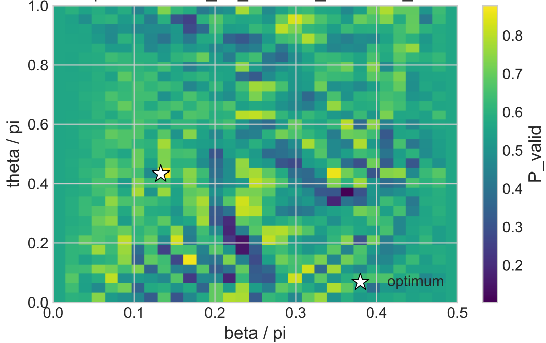
V5 P_valid heatmap at r=45 - 08_2d_medium_clustered_obstacles - descent
