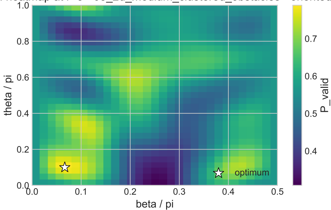
V5 P_valid heatmap at r=3 - 08_2d_medium_clustered_obstacles - oriented_valid
