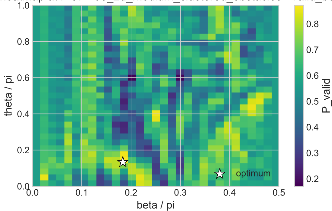
V5 P_valid heatmap at r=37 - 08_2d_medium_clustered_obstacles - valid_boundary
