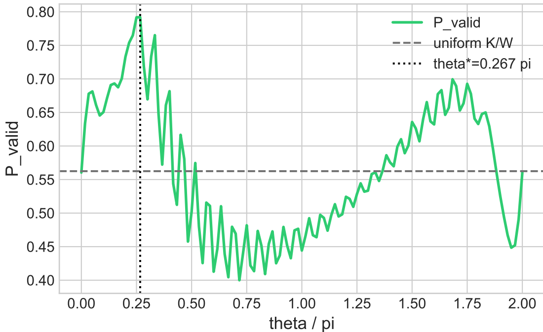
V5 theta scan at beta=0.220, r=37 - valid_boundary
