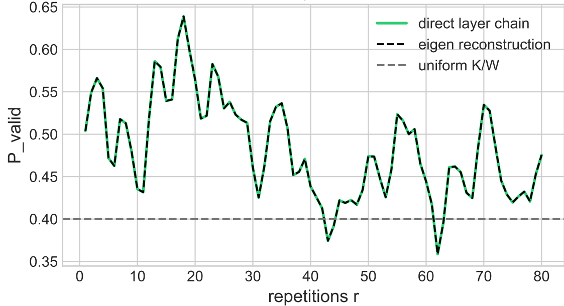
Period prediction
