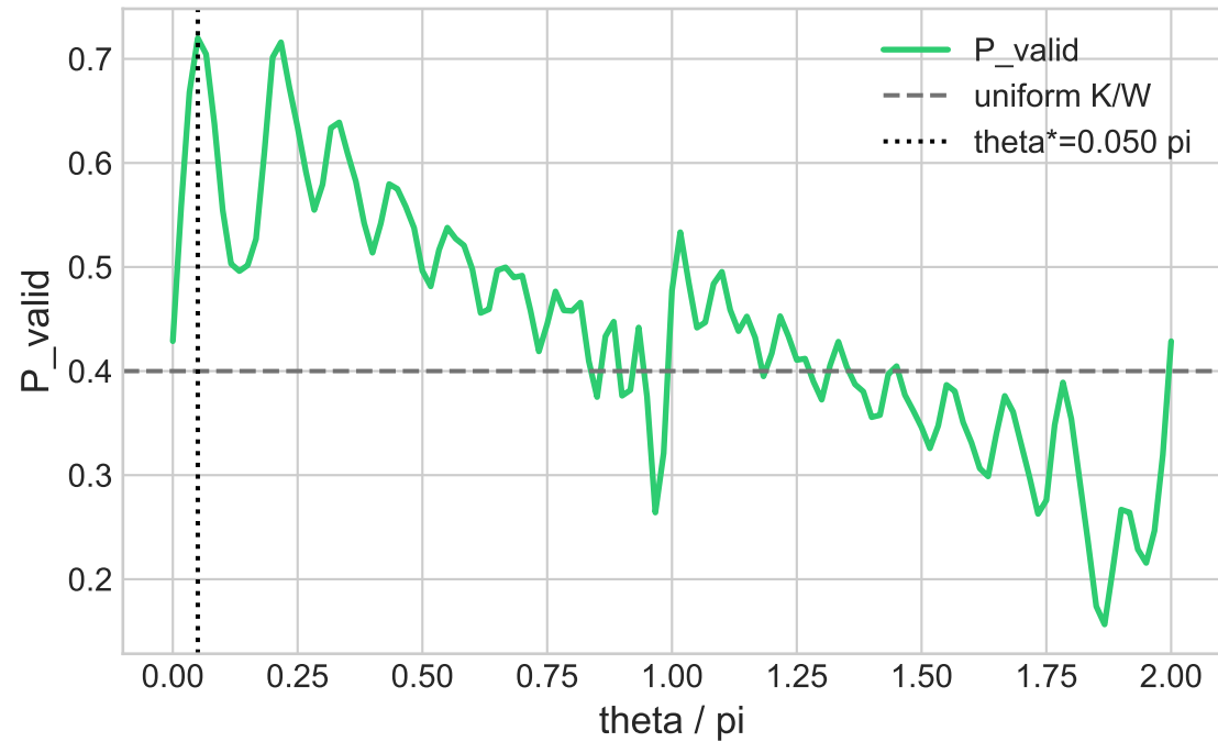
V5 theta scan at beta=0.180, r=18 - descent
