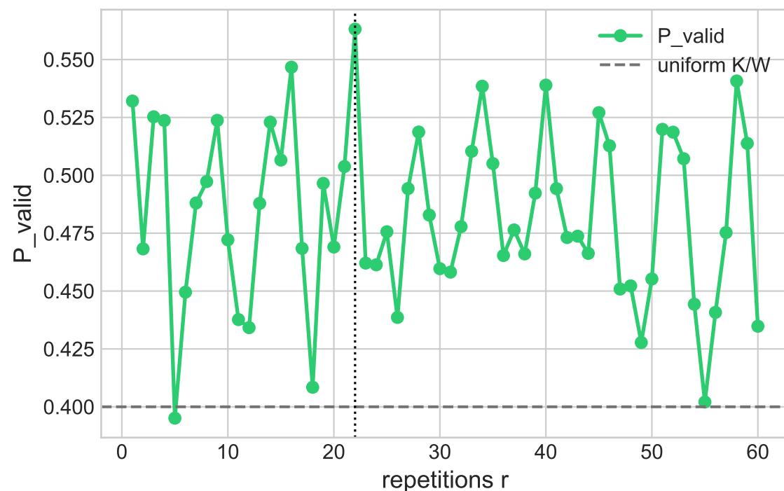
Theta scan
