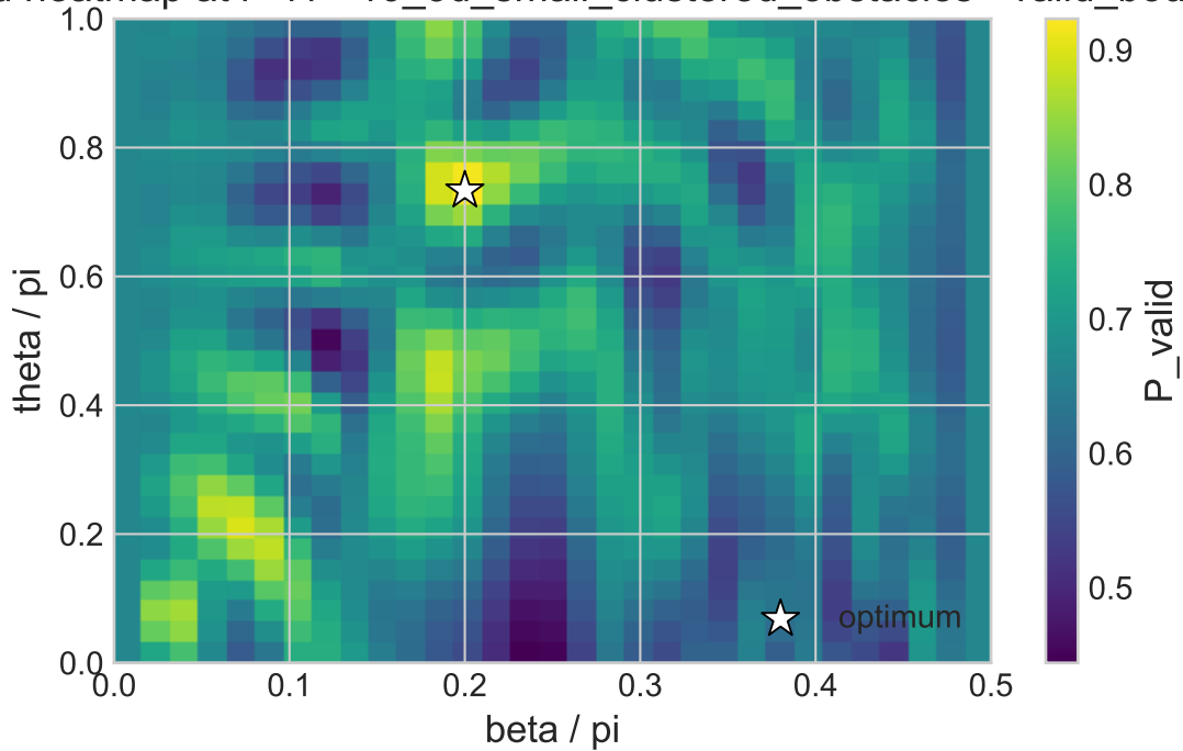
V5 P_valid heatmap at r=11 - 10_3d_small_clustered_obstacles - valid_boundary
