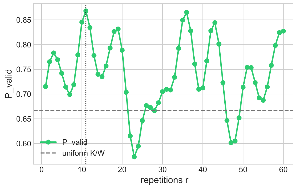
Theta scan
