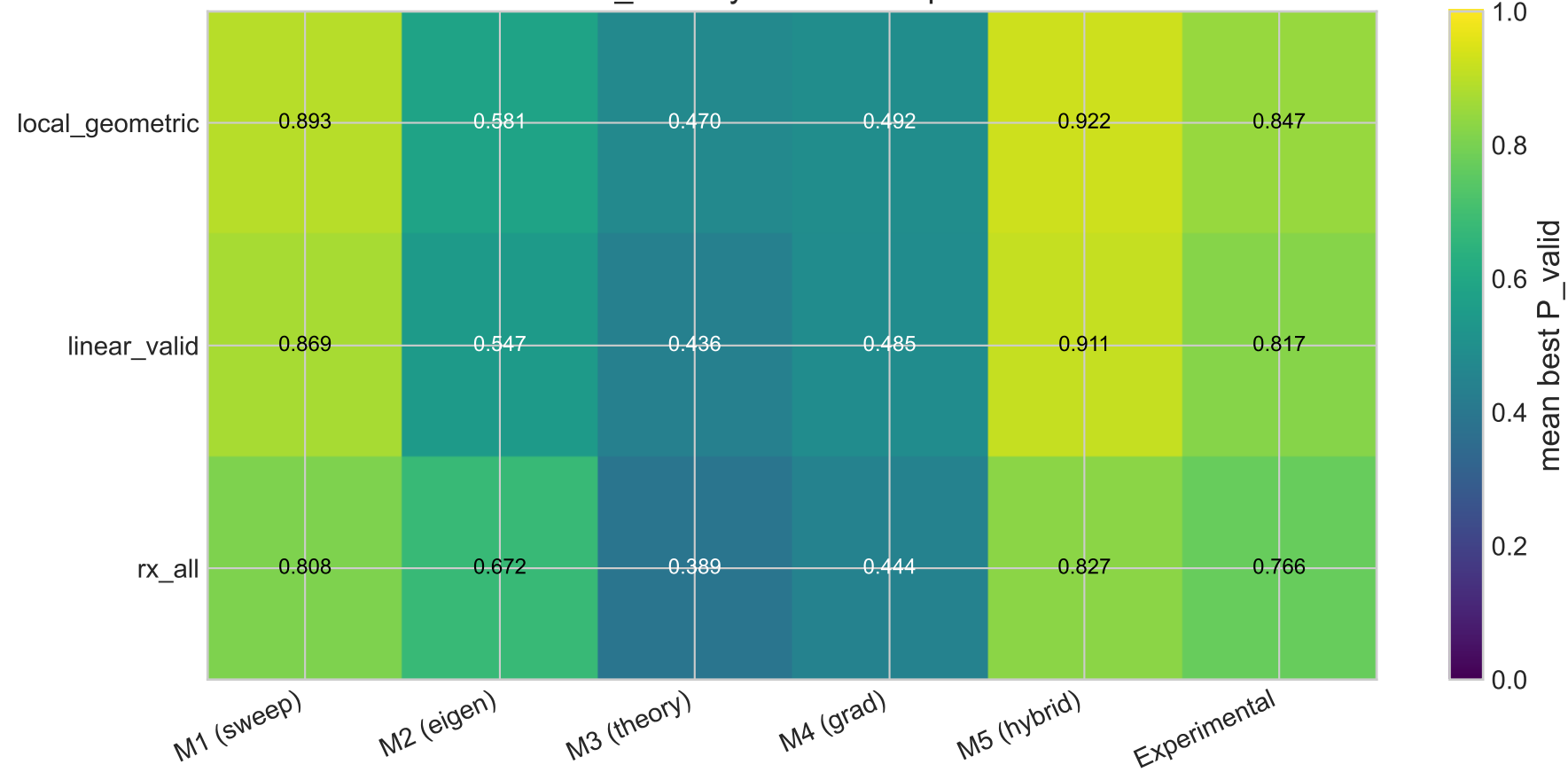
V5 mean best P_valid by mixer and optimization method
