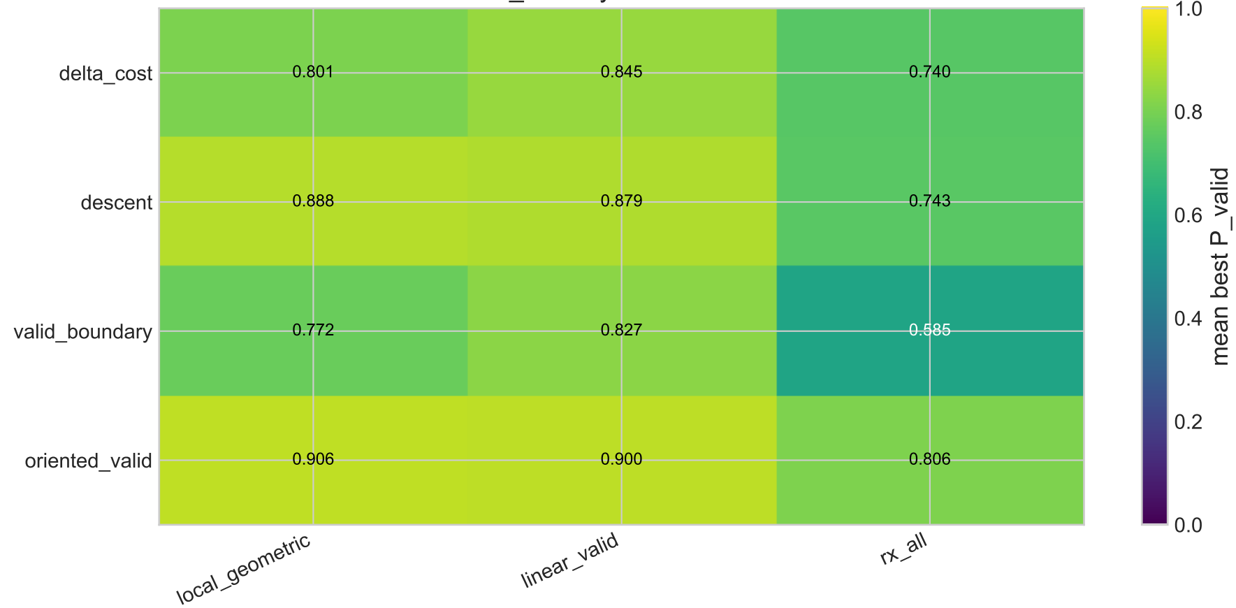
V5 mean best P_valid by transition mode and mixer
