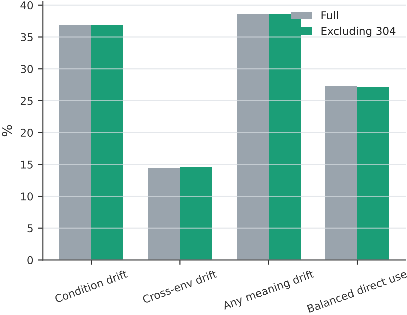
D Sensitivity: excluding 304 rows
