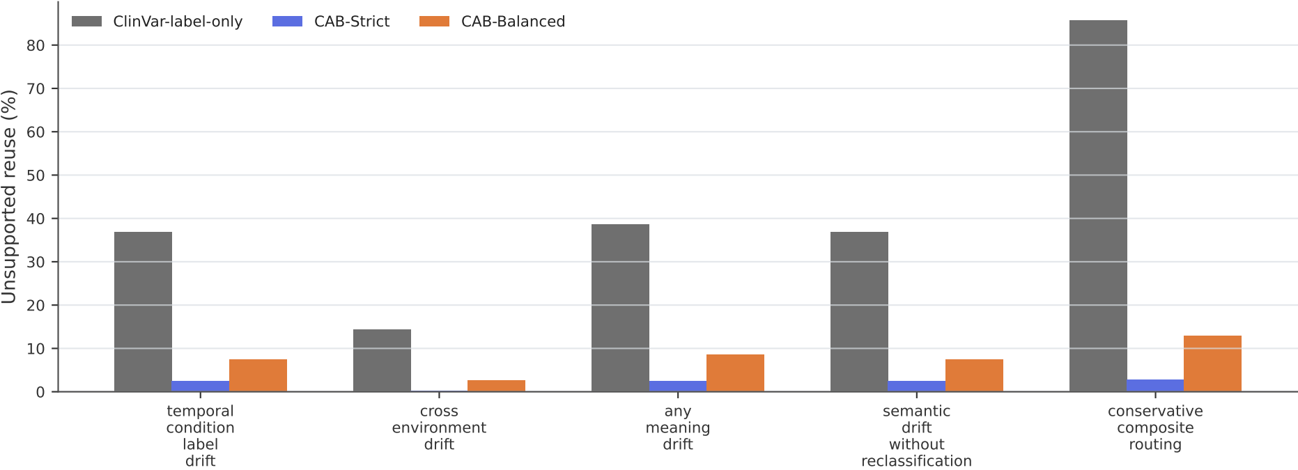
Unsupported reuse by endpoint and mode
