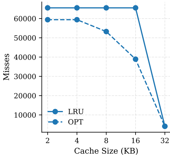
Transpose
