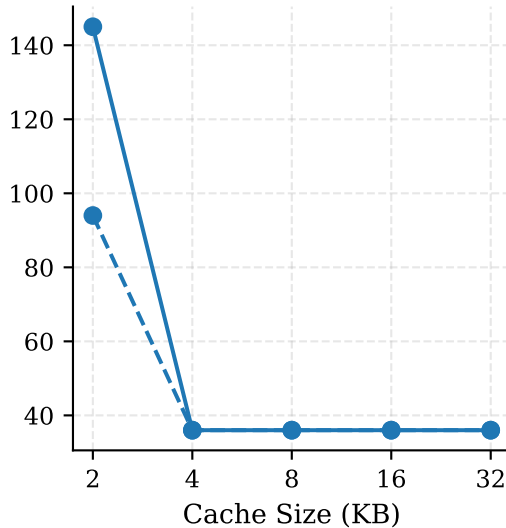
Gather
