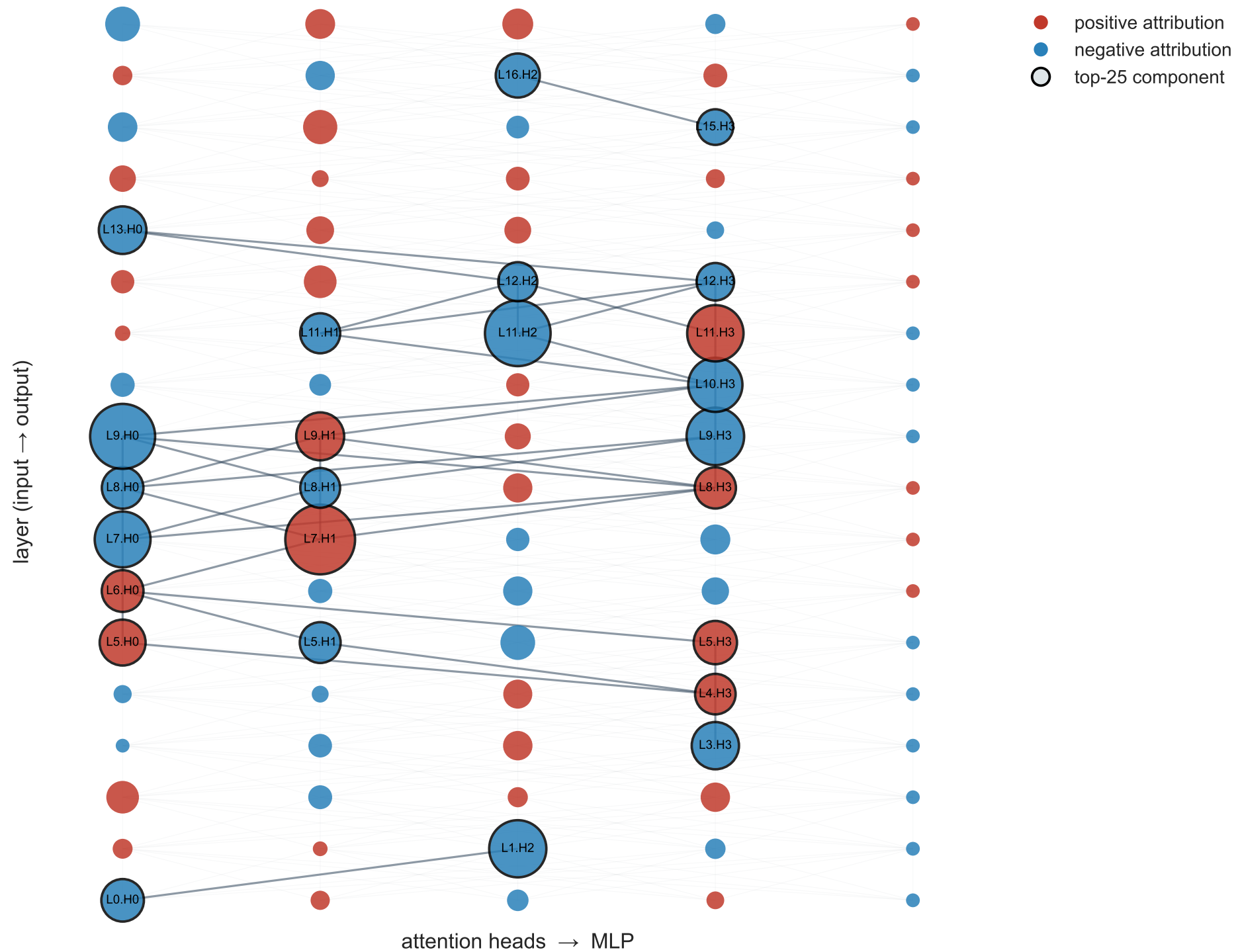
functiongemma-270m-it_tool_selection_int4
