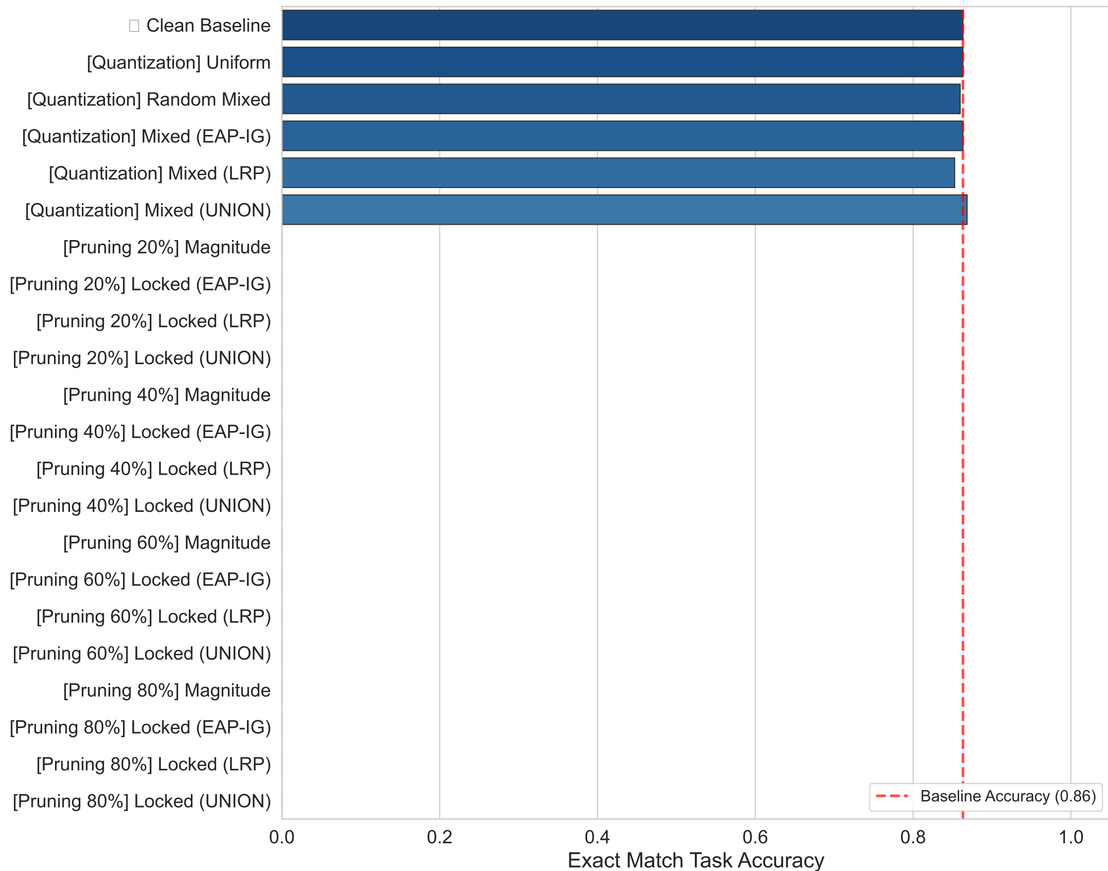
Comprehensive Accuracy Breakdown: ioi
