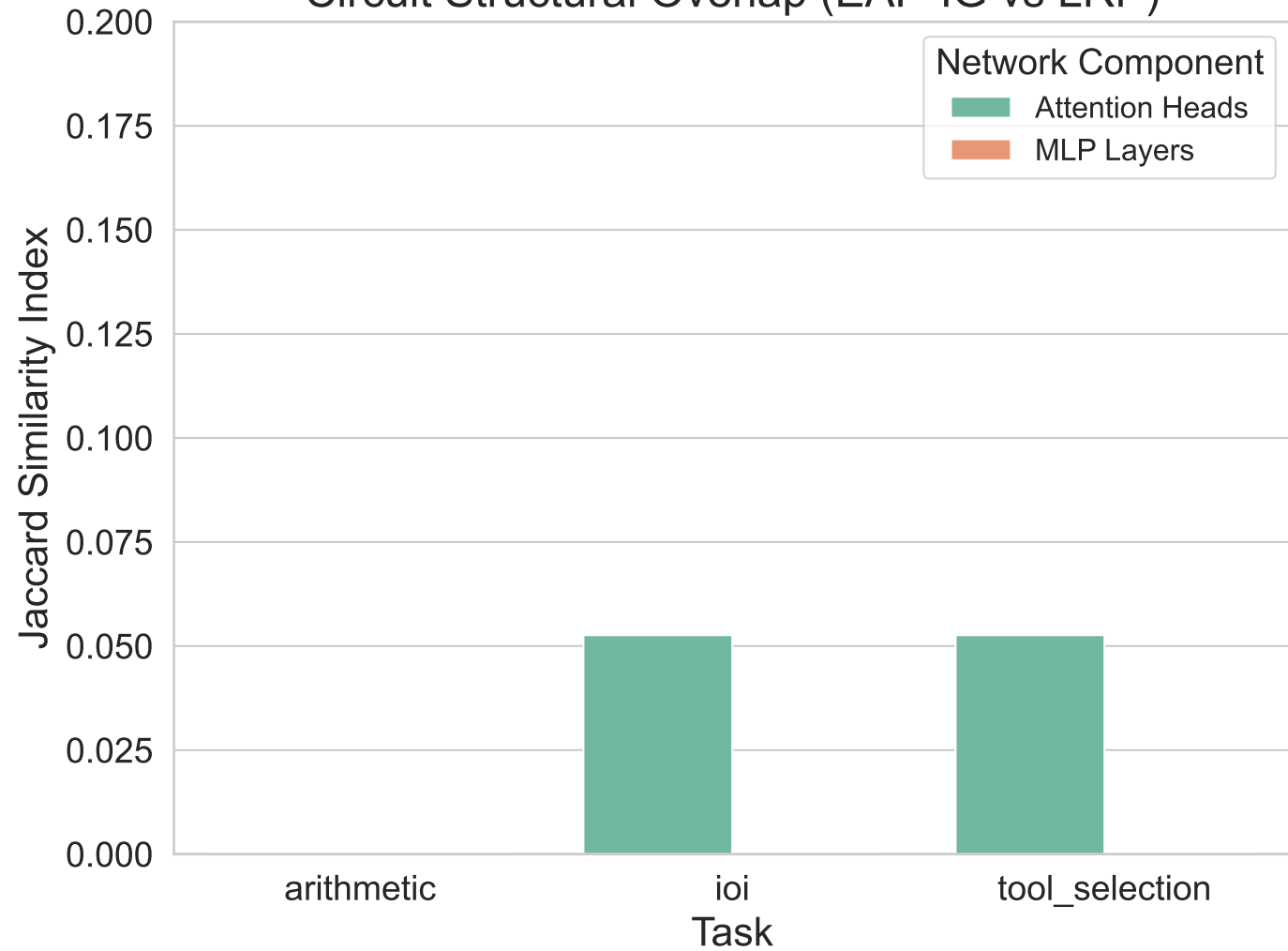
Circuit Structural Overlap (EAP-IG vs LRP)
