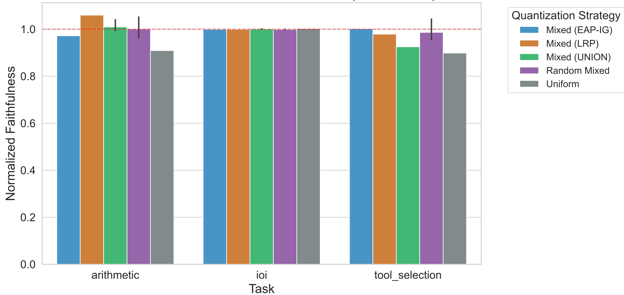
Mixed-Precision Quantization vs. Uniform (Faithfulness)
