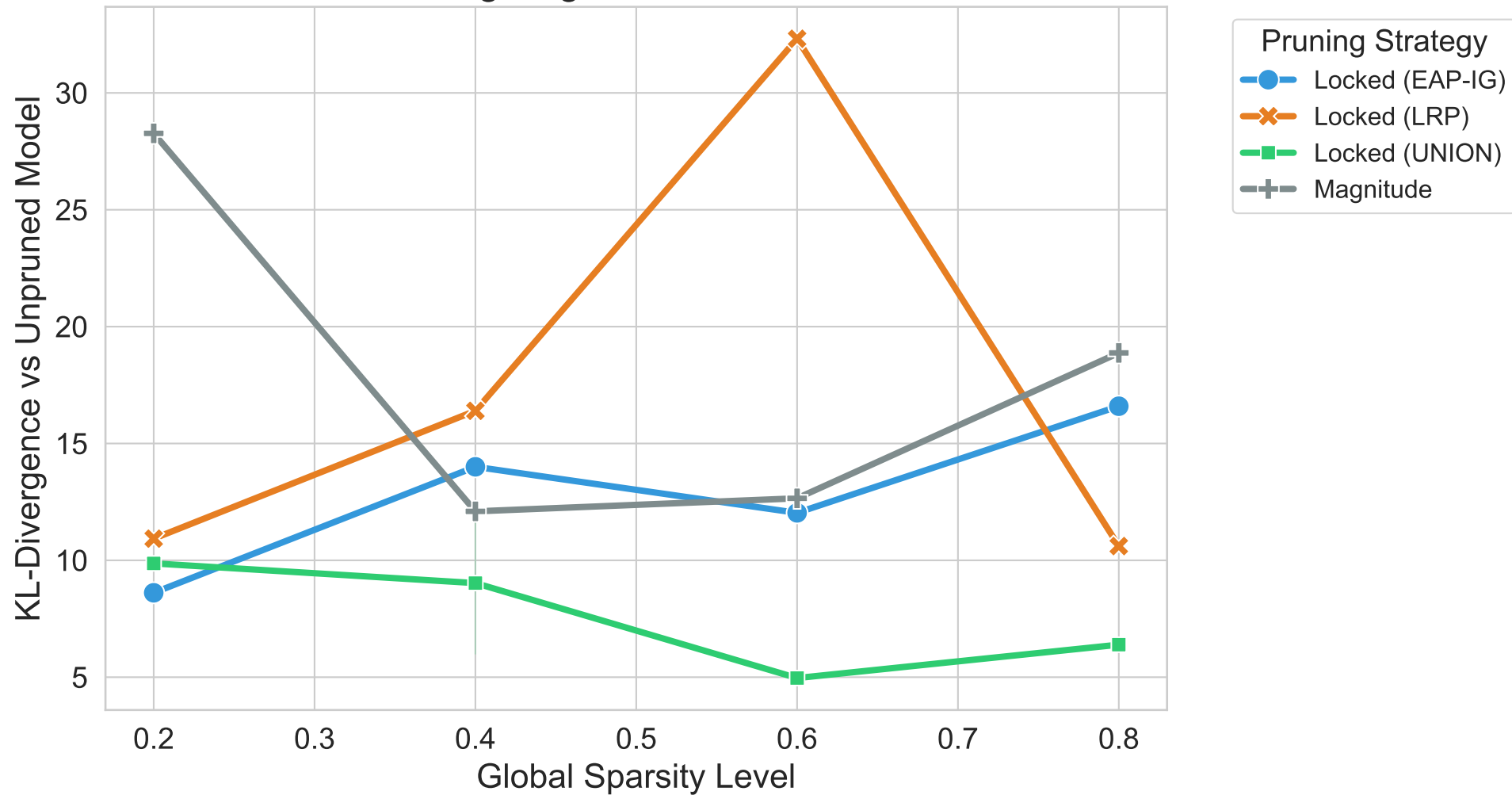
Pruning Degradation: arithmetic
