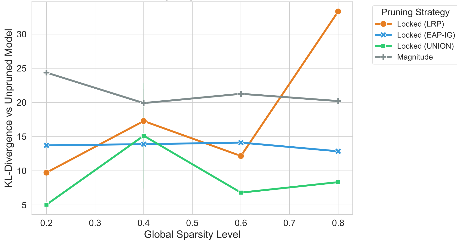
Pruning Degradation: ioi
