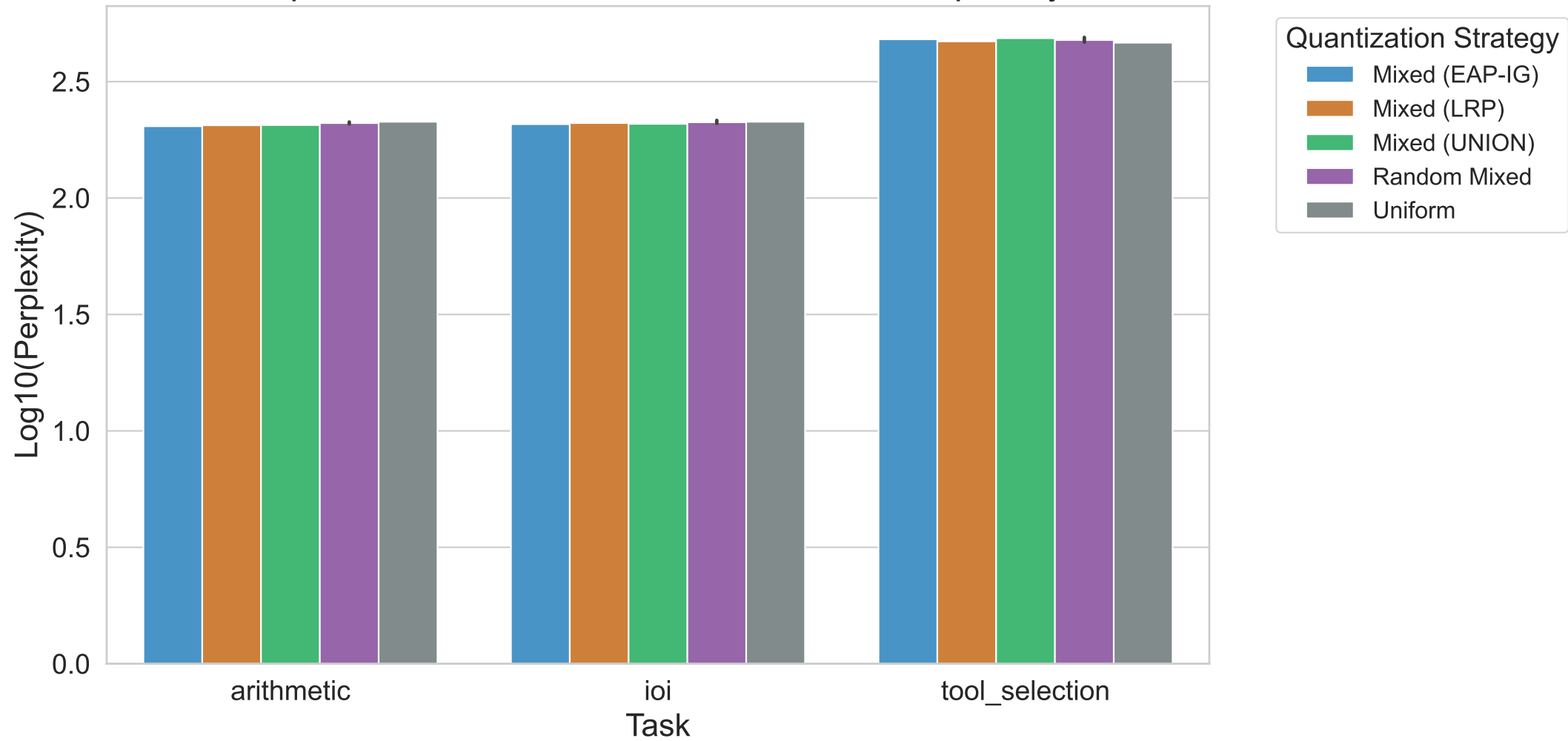
Impact of Quantization on General Model Capability
